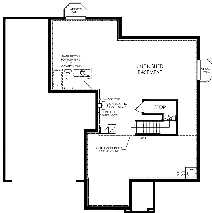
UNFINISHED BASEMENT FLOOR
