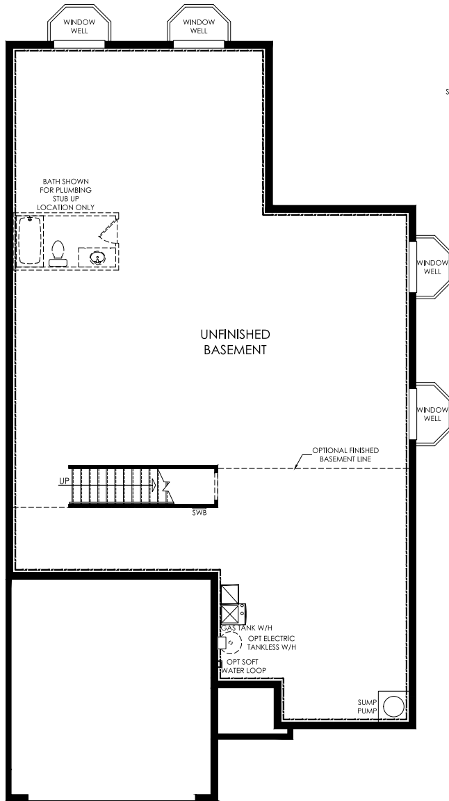
UNFINISHED BASEMENT FLOOR
