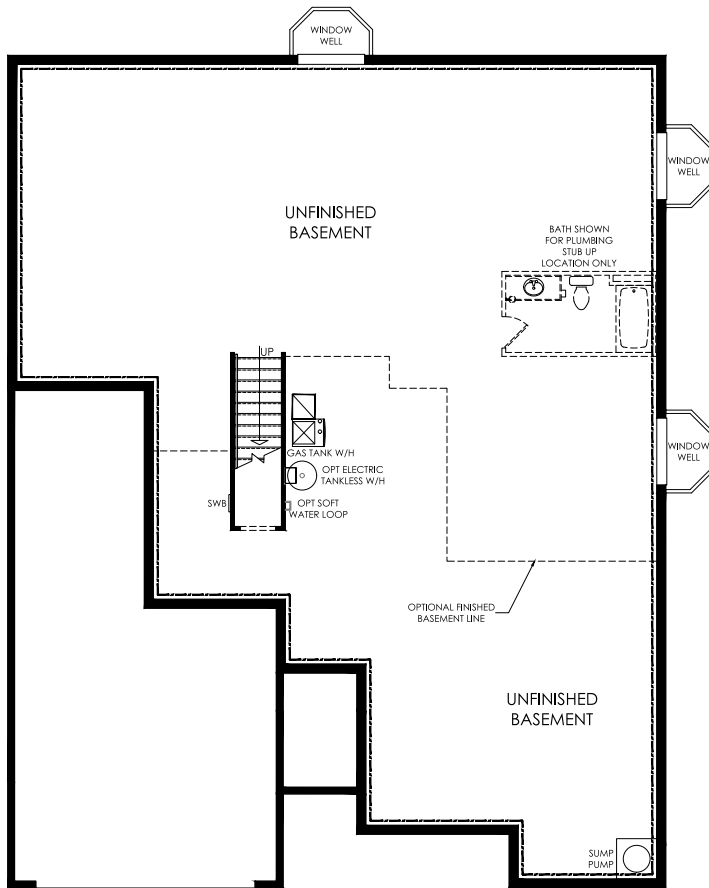
UNFINISHED BASEMENT FLOOR
