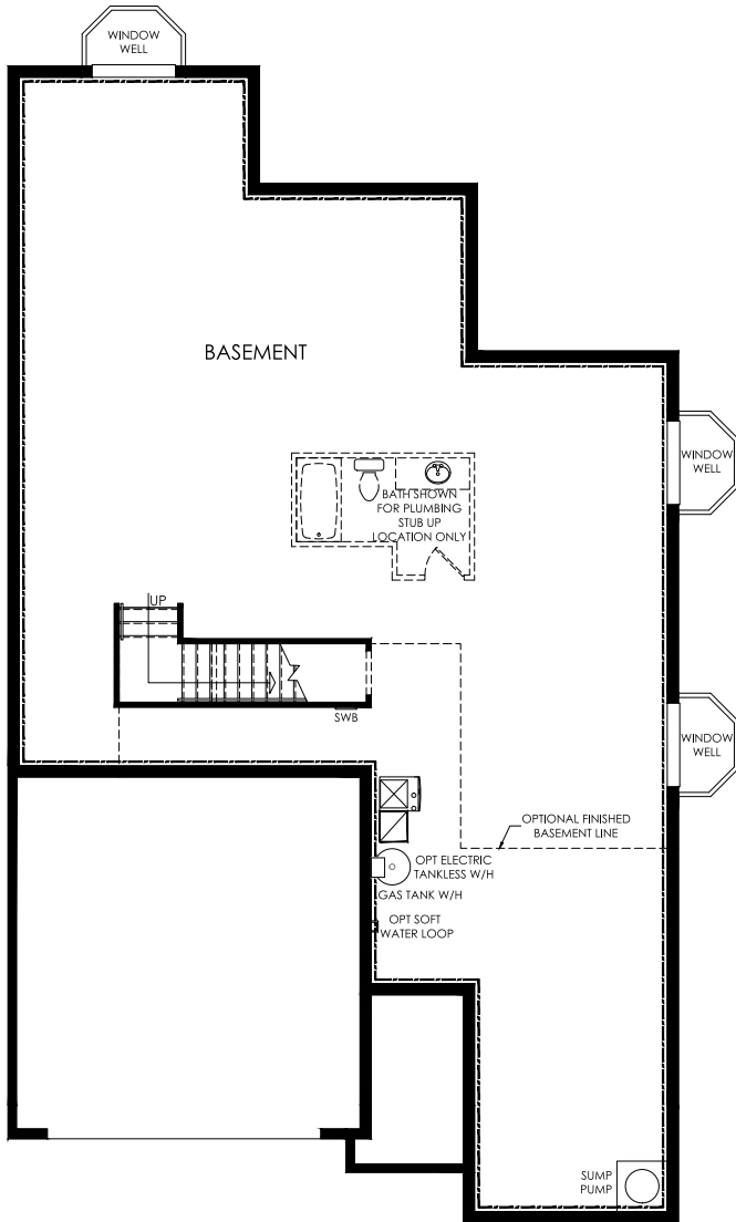
UNFINISHED BASEMENT FLOOR
